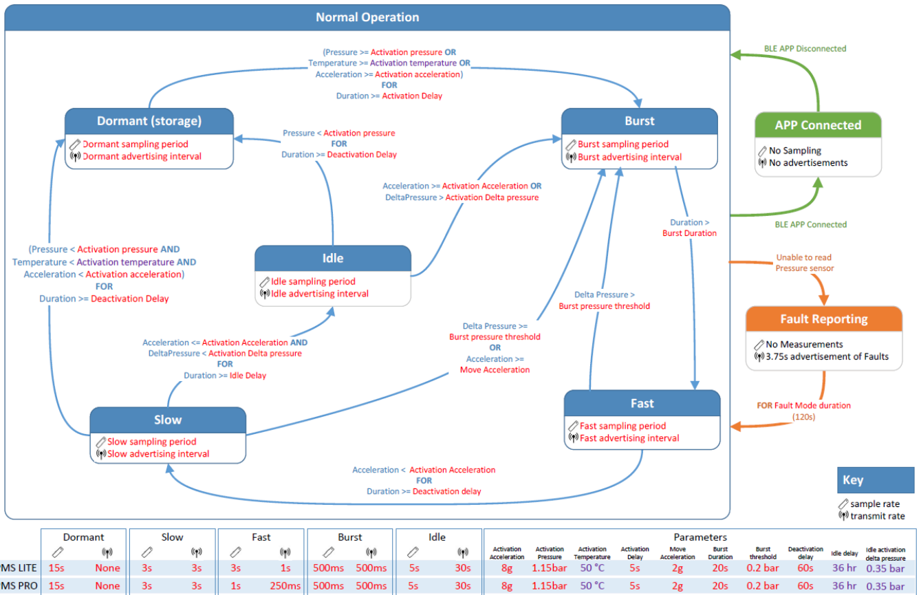
Figure 20 - IRTPMS v1.7 state diagram
