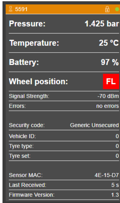
Figure 94 - Default FL sensor
