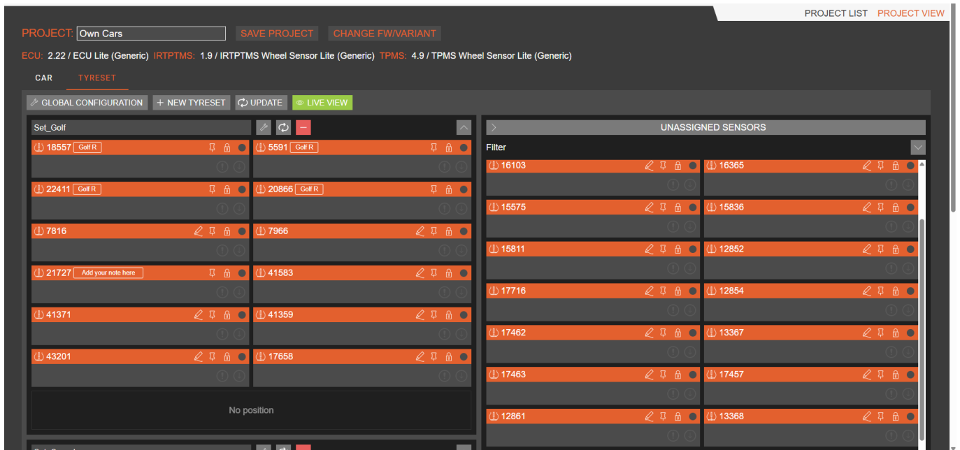
Figure 113 - Batch update
