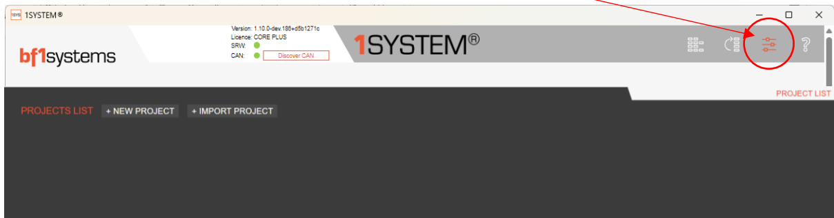
Figure 101 - Projects page
