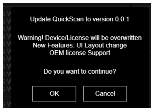
Figure 135 - Quickscan update
