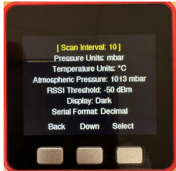
Figure 139 - Settings
