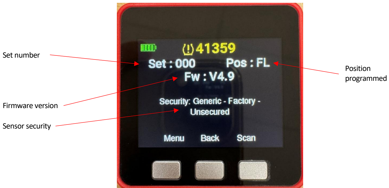
Figure 137 - More screen
