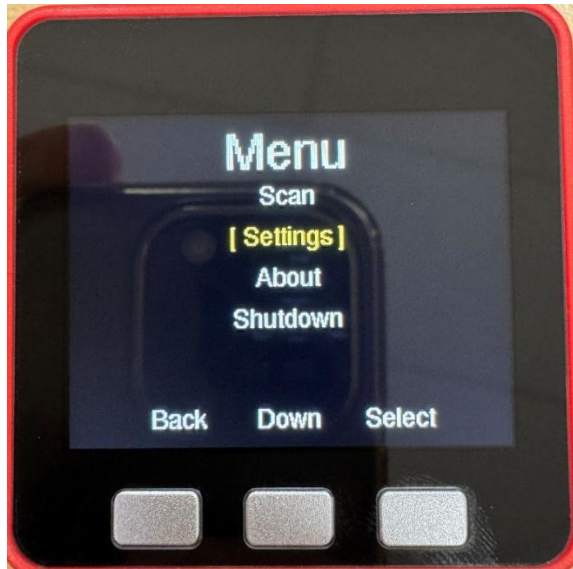
Figure 138 - Menu screen
