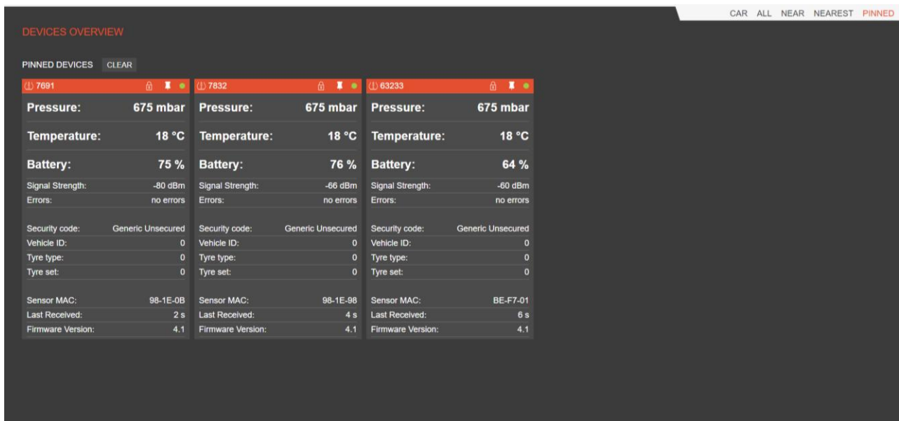
Figure 84 - Pinned sensors
