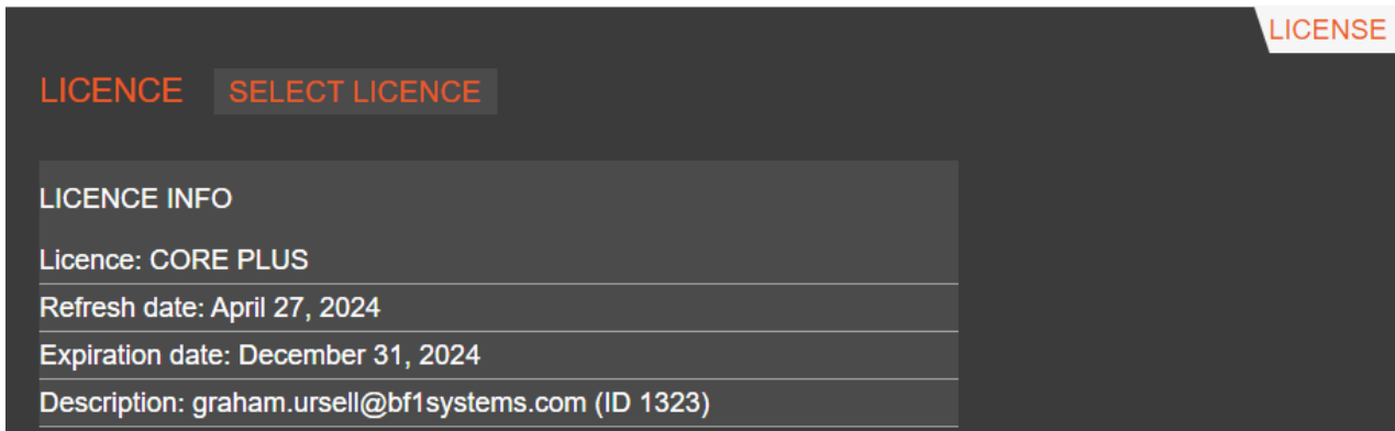
Figure 11 - Licence remaining
