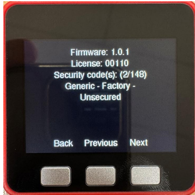
Figure 140 - About screen
