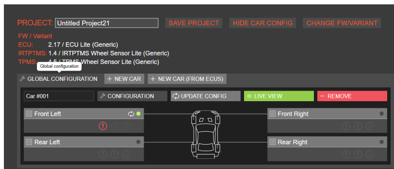
Figure 114 - Global configuration button
