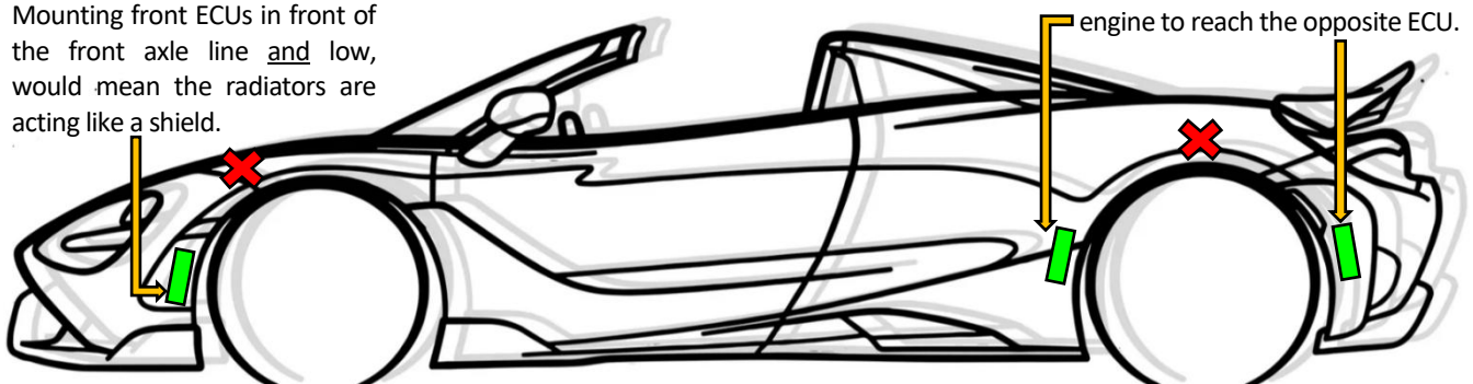
Figure 25 - Examples of ECU mounting positions
