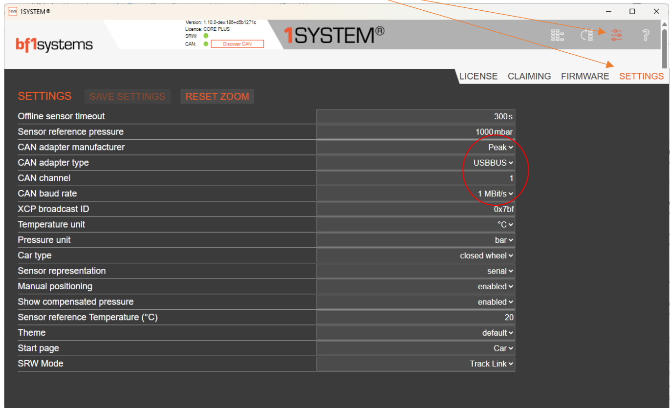
Figure 5 - CAN settings
