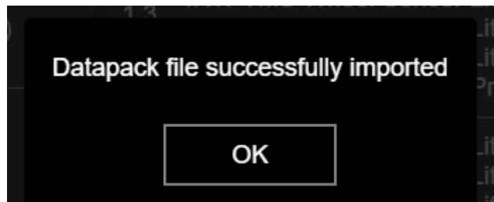
Figure 90 - Datapack imported
