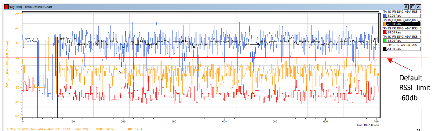
Figure 116 - RSSI of each sensor received by the ECU
