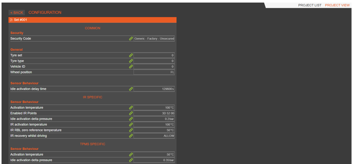
Figure 111 - Global tyre settings
